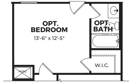
Partial First Floor Plan @ Opt. Bedroom
