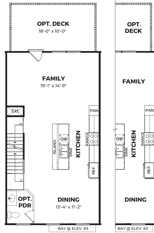
Second Floor Plan @ Mid-Kitchen
