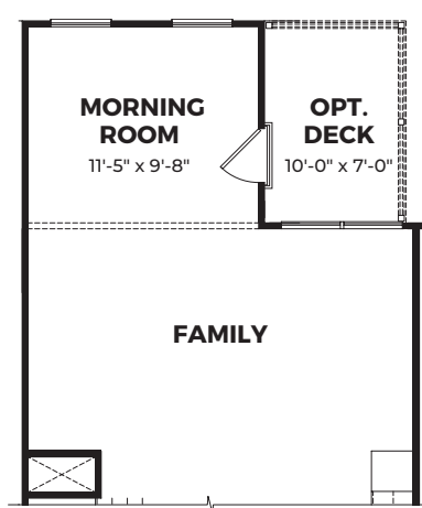
Second Floor Plan @ Opt. Morning Room w/ Mid-Kitchen
