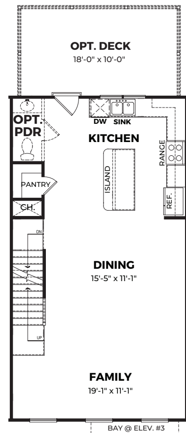
Second Floor Plan @ Rear-Kitchen
